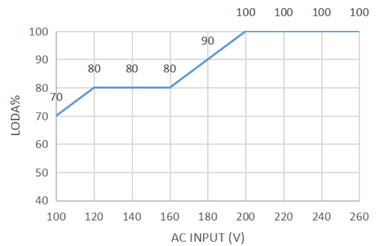
Static Characteristics Curve (Load vs. Input Voltage)
