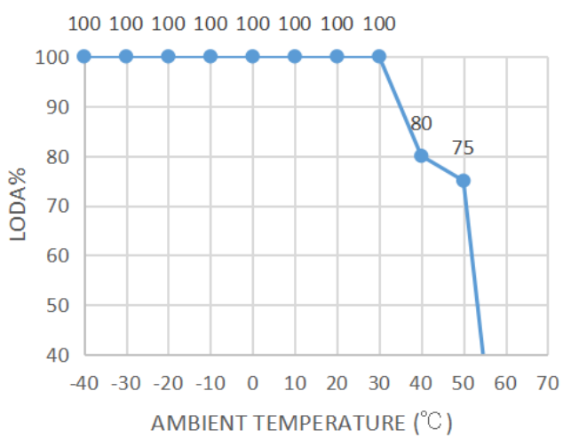
Derating Curve vs Ambient Temperature
